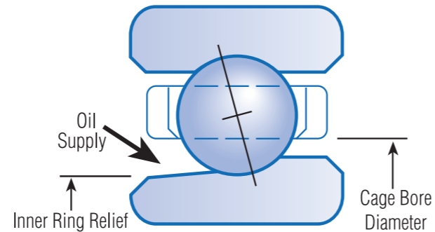
Fig. 17. Lubrication window for B-type bearings.
