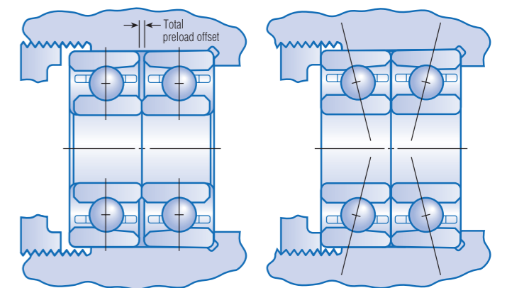
Fig. 9. DF mounting.
