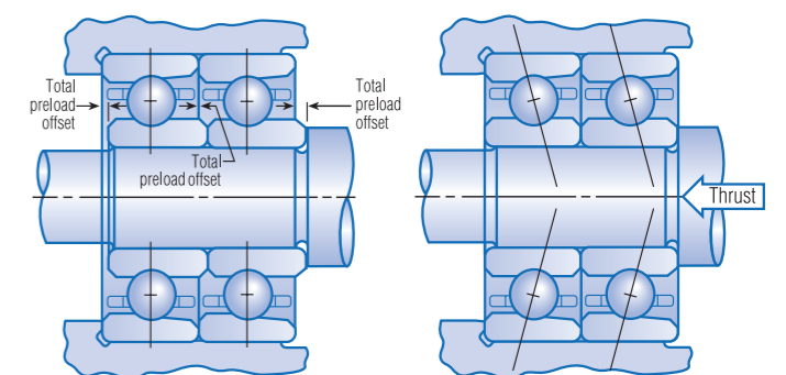
Fig. 10. DT mounting.
