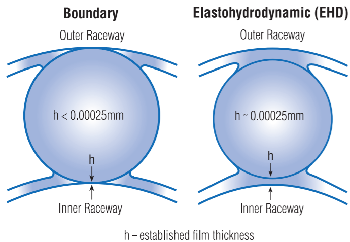
Fig. 13. Lubrication Regimes.
