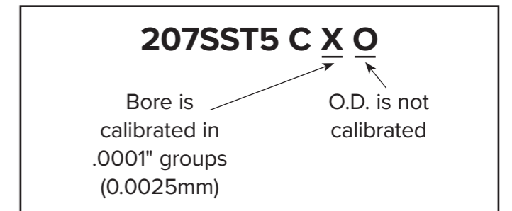
Fig. 22. Example of random calibration nomenclature.
