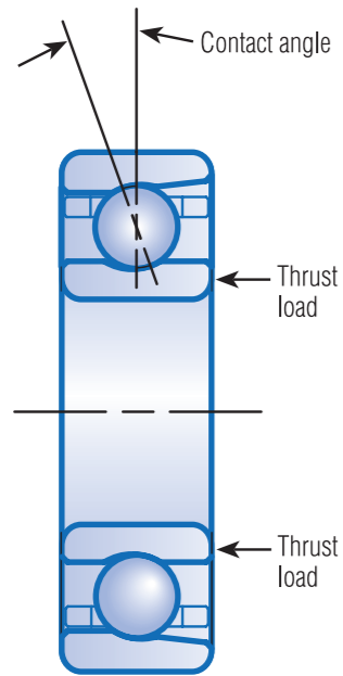
Fig. 4. Contact angle refers to the nominal angle between the ball-to-race contact line and a plane through the ball centres, perpendicular to the bearing axis.
