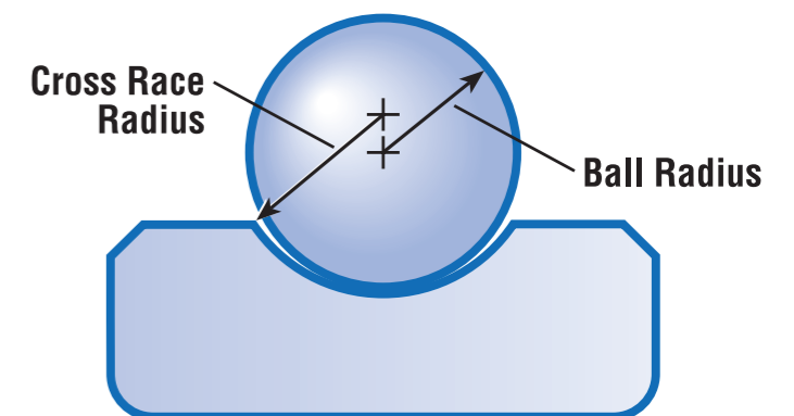
Fig. 2. Raceway curvature.
