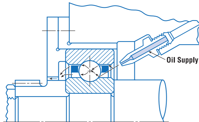
Fig. 15. Jet lubrication system.
