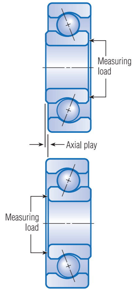
Fig. 5. Axial play, or end play, is defined as the maximum possible movement, parallel to the axis of the bearing, of the inner ring relative to the outer ring.
