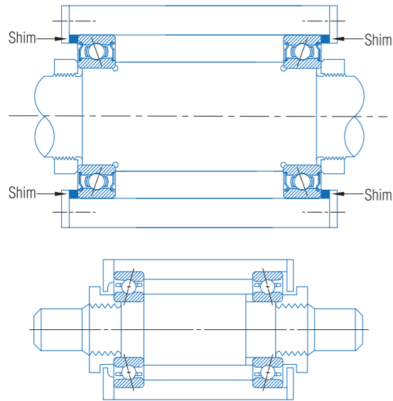
Fig. 7. Axial adjustment.
