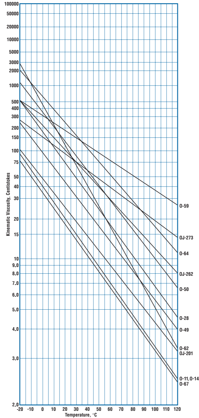
Viscosity graph for several typical oil lubricants.
