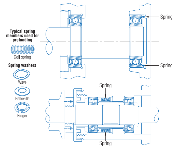
Fig. 6. Different types of spring preloading.
