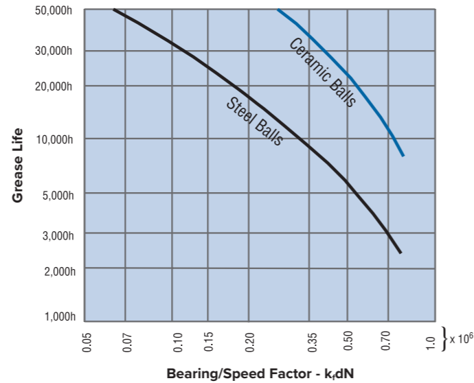
Fig. 20. Grease life computation for normal temperatures.
