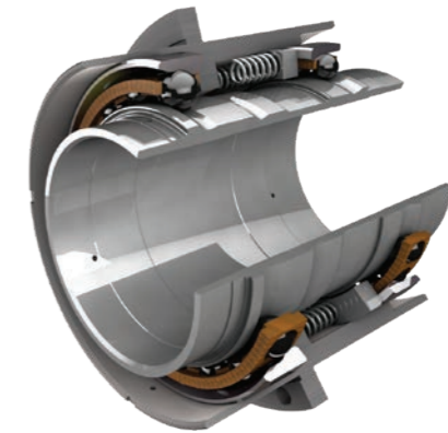
Special double row assembly with integrated housing for large general vacuum pump
