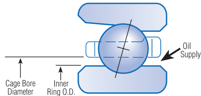
Fig. 17. Lubrication window for B-type bearings.
