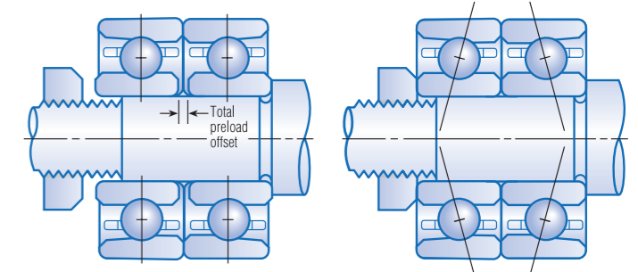
Fig. 8. DB mounting.
