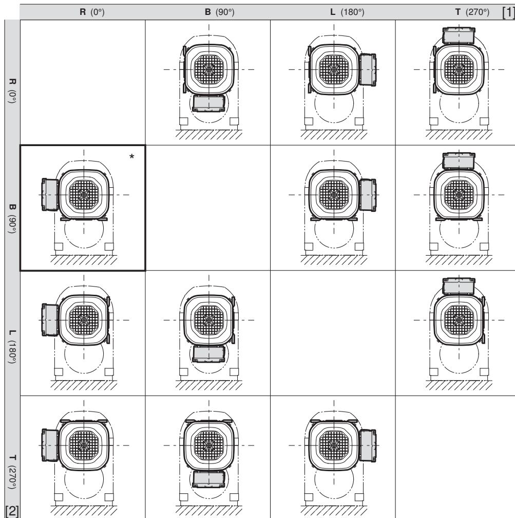
[1] Terminal box positions
