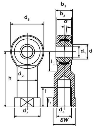
SI..K SS Internal Thread
