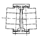
Angular Misalignment
