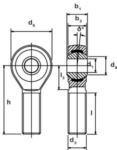
SA..K SS External Thread
